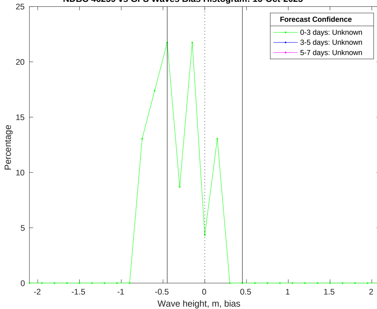
NDBC 46259 vs GFS Waves Bias Histogram: 16-Oct-2025
