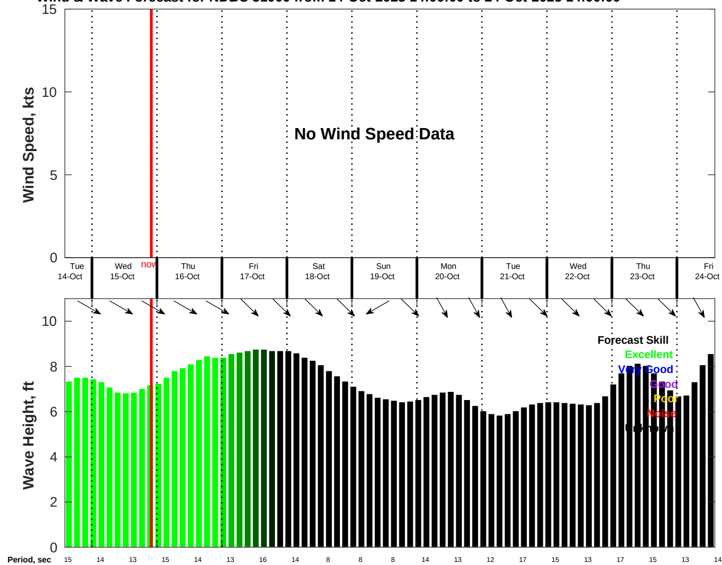
Wind & Wave Forecast for NDBC 51000 from 14-Oct-2025 14:00:00 to 24-Oct-2025 14:00:00
