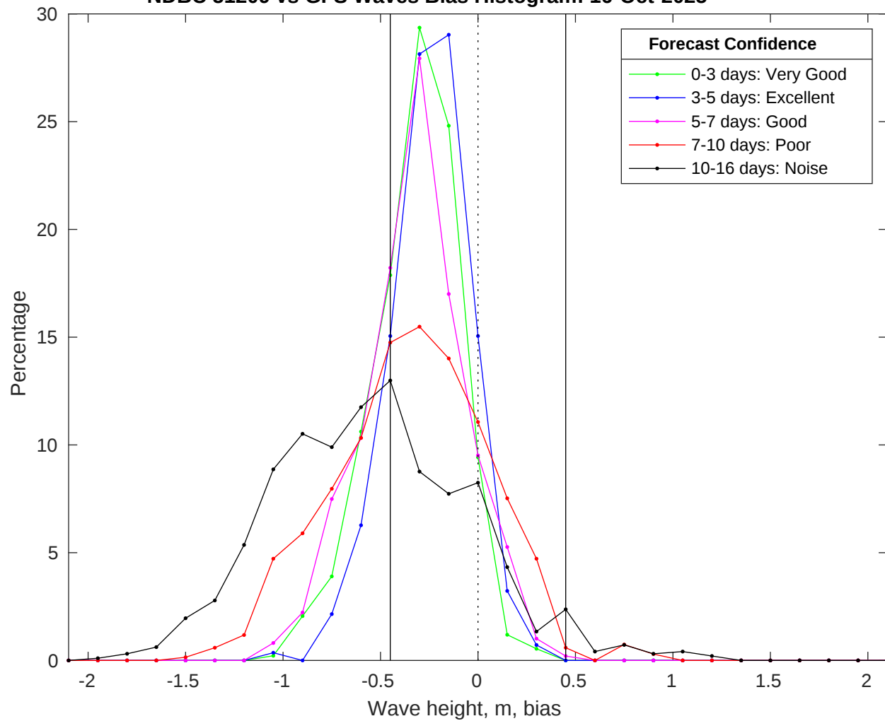
NDBC 51209 vs GFS Waves Bias Histogram: 16-Oct-2025
