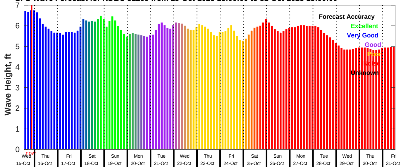
GFS Wave Forecast for NDBC 51209 from 15-Oct-2025 13:00:00 to 31-Oct-2025 13:00:00
