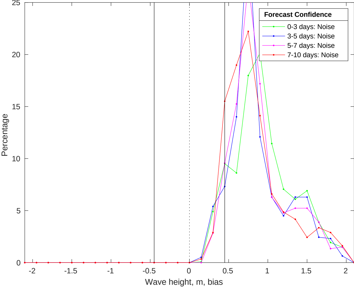
NDBC 51211 vs CMEMS Waves Bias Histogram: 16-Oct-2025
