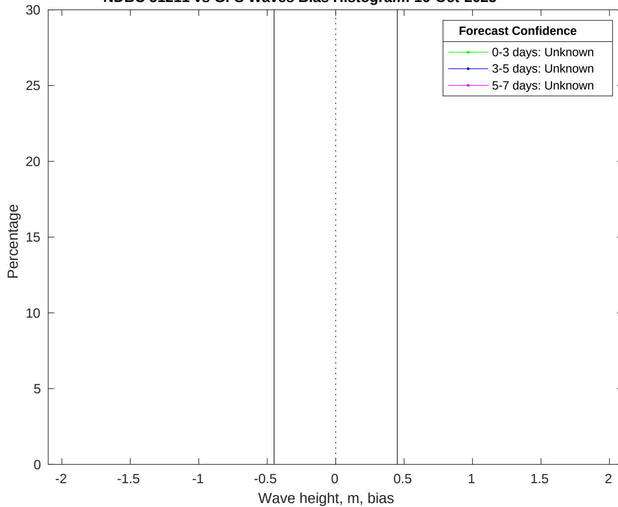
NDBC 51211 vs GFS Waves Bias Histogram: 16-Oct-2025
