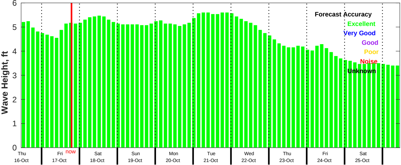
CMEMS Wave Forecast for NDBC 52211 from 15-Oct-2025 11:00:00 to 25-Oct-2025 11:00:00
