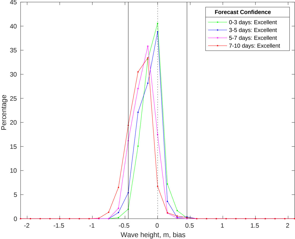
NDBC 52213 vs CMEMS Waves Bias Histogram: 16-Oct-2025
