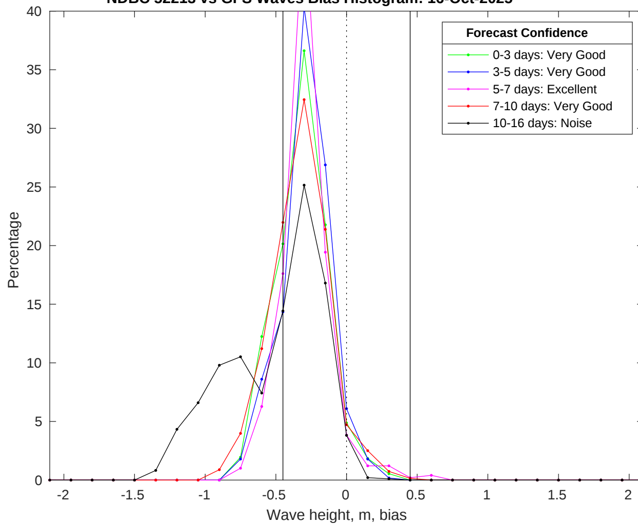
NDBC 52213 vs GFS Waves Bias Histogram: 16-Oct-2025
