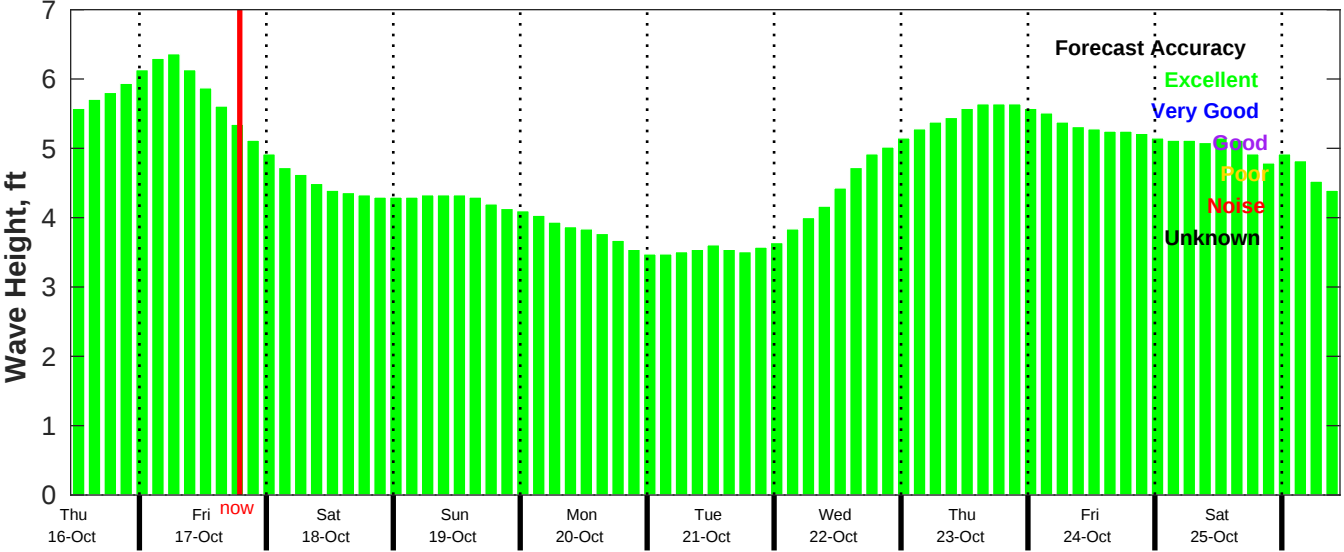
CMEMS Wave Forecast for NDBC 52213 from 15-Oct-2025 11:00:00 to 25-Oct-2025 11:00:00
