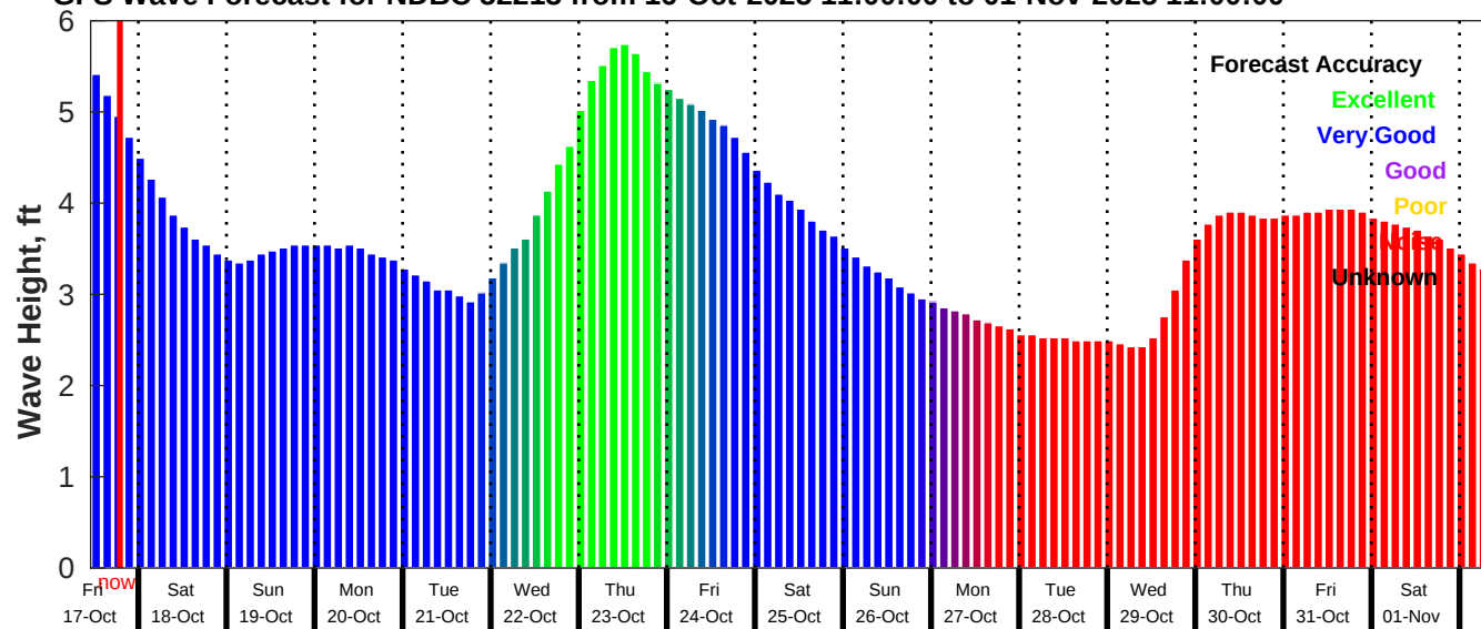
GFS Wave Forecast for NDBC 52213 from 16-Oct-2025 11:00:00 to 01-Nov-2025 11:00:00
