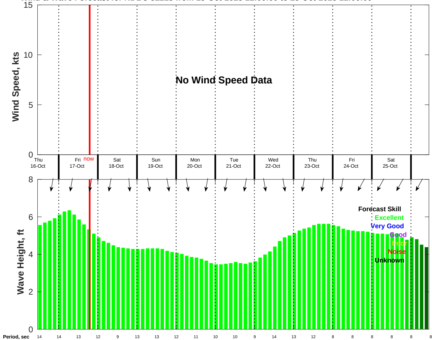
Wind & Wave Forecast for NDBC 52213 from 15-Oct-2025 11:00:00 to 25-Oct-2025 11:00:00
