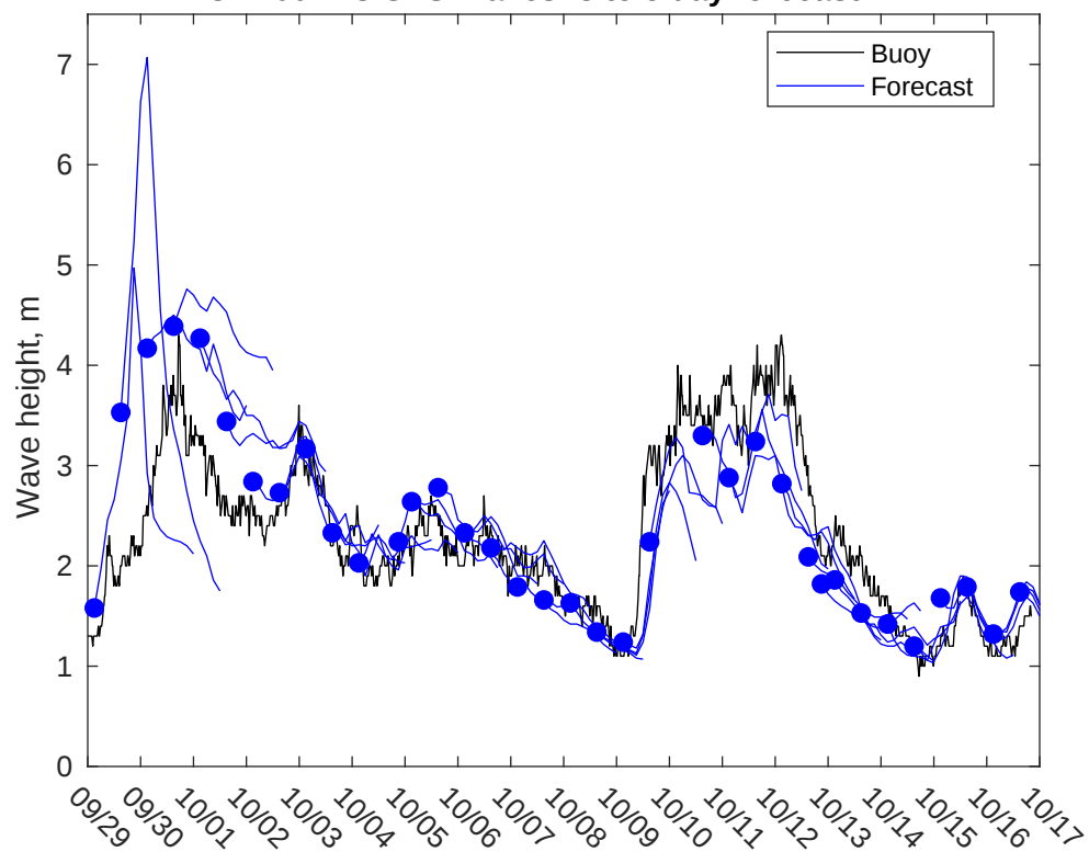
NDBC 41004 vs GFS Waves: 3 to 5 day forecast
