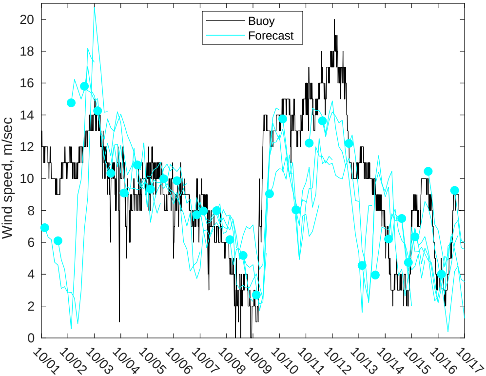
NDBC 41004 vs GFS Winds: 5 to 7 day forecast
