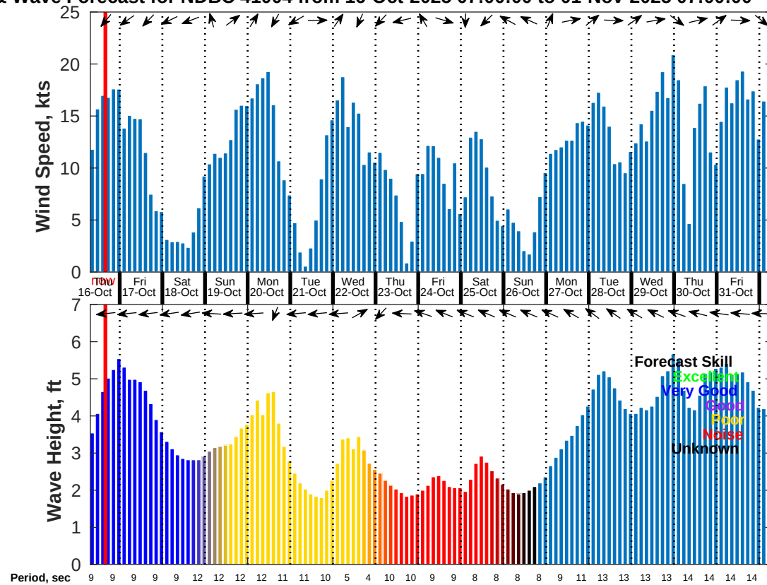
Wind & Wave Forecast for NDBC 41004 from 16-Oct-2025 07:00:00 to 01-Nov-2025 07:00:00
