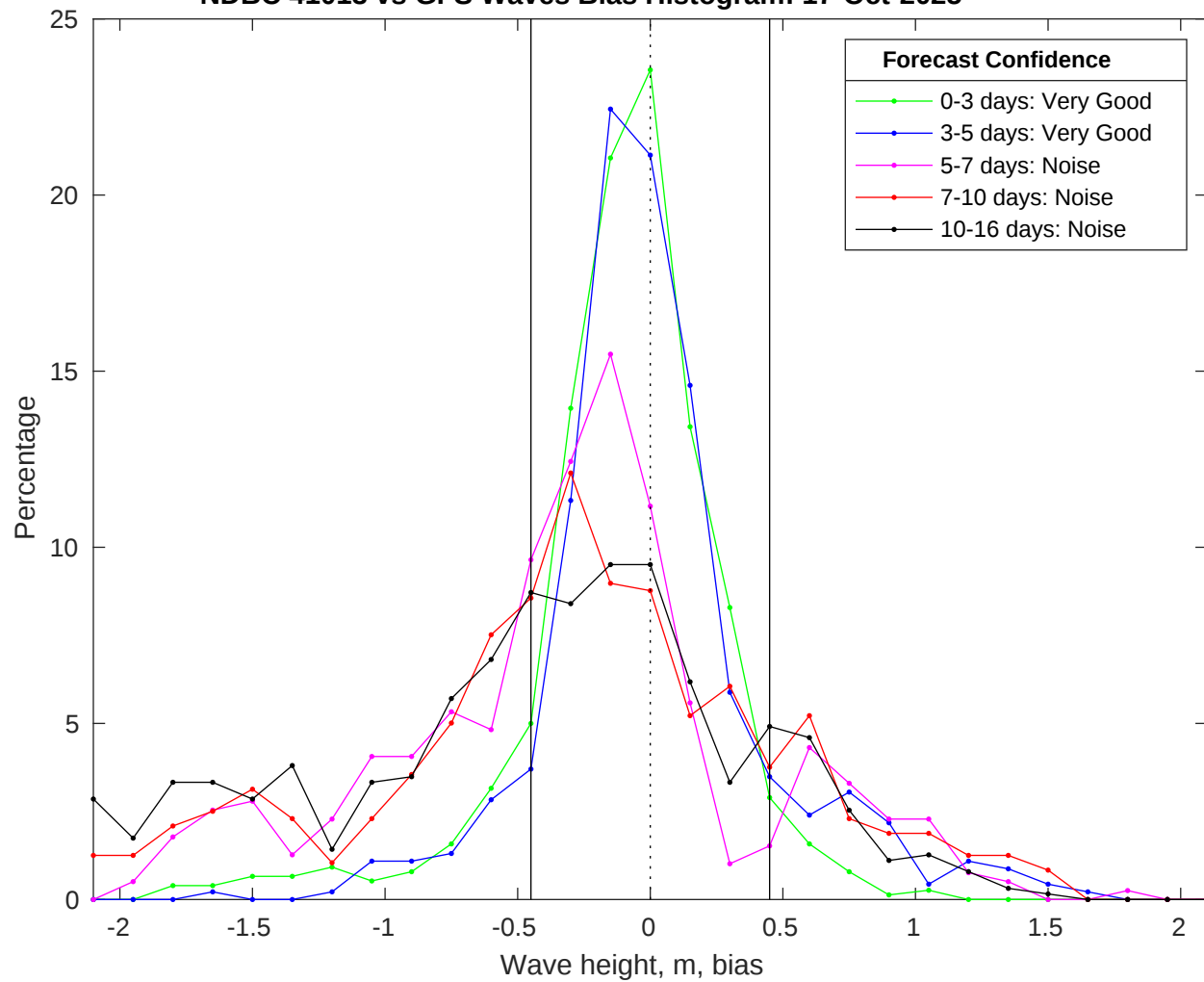
NDBC 41013 vs GFS Waves Bias Histogram: 17-Oct-2025
