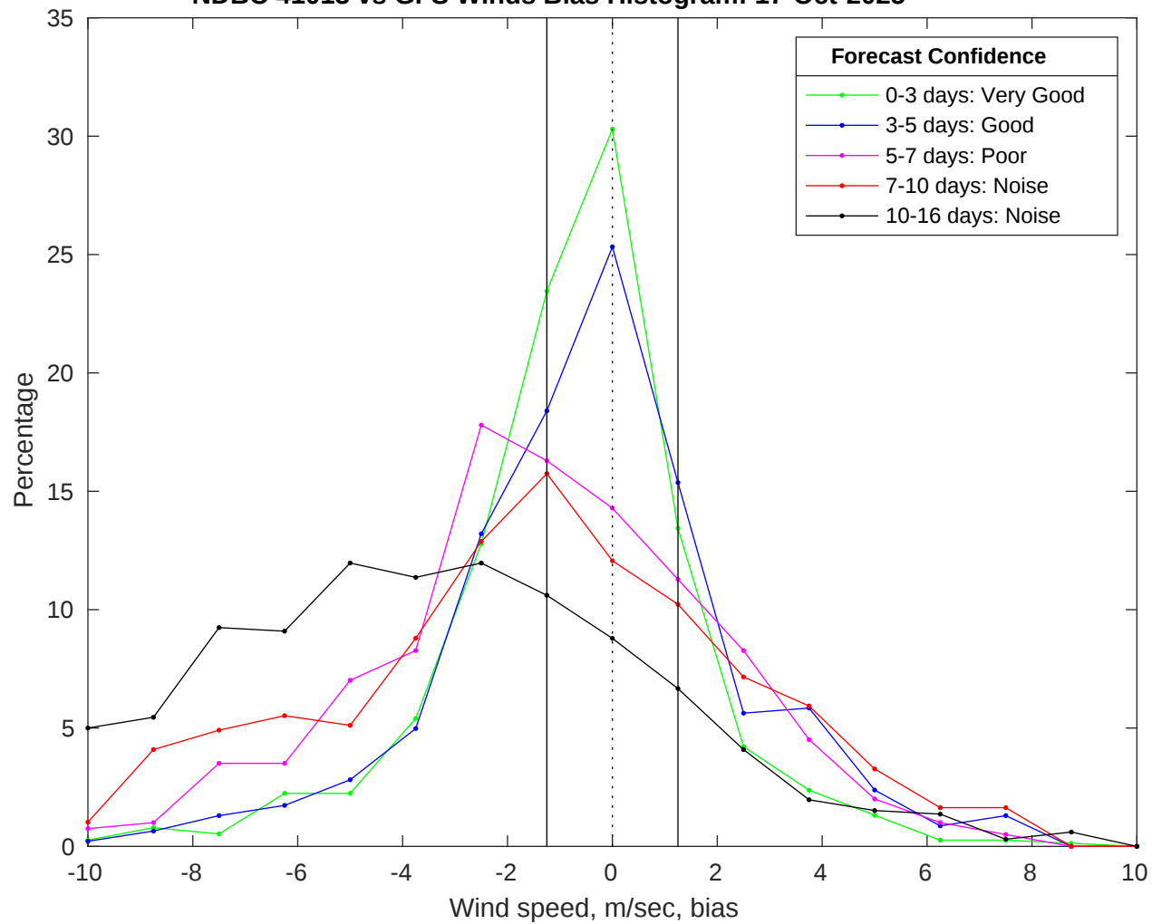
NDBC 41013 vs GFS Winds Bias Histogram: 17-Oct-2025
