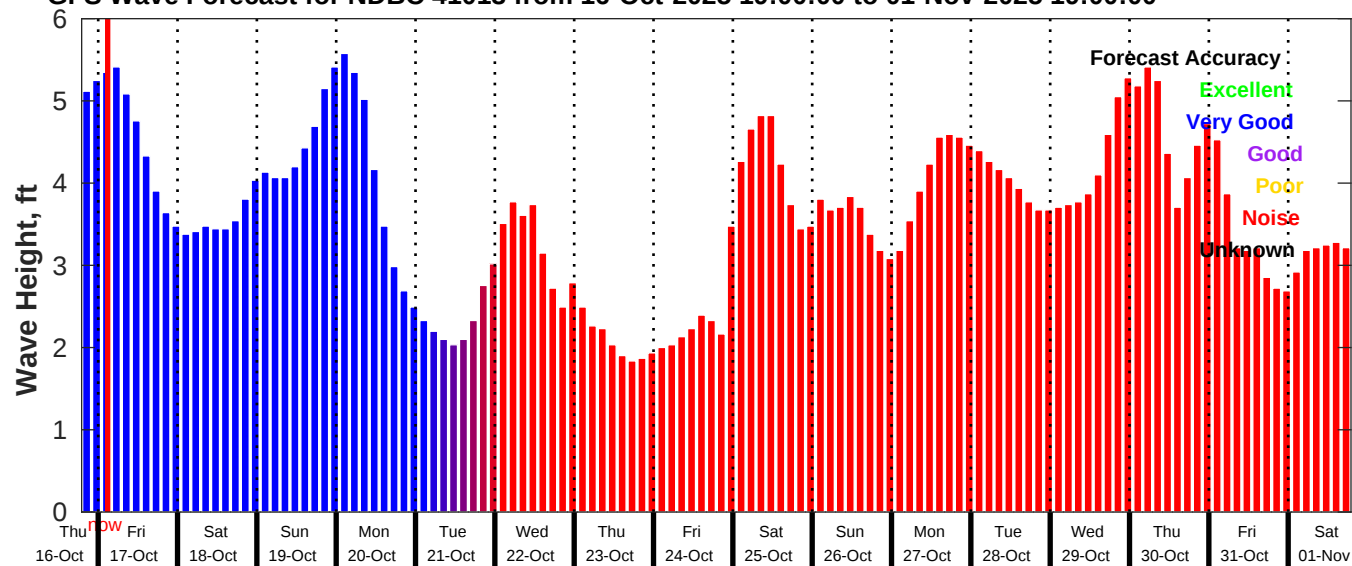
GFS Wave Forecast for NDBC 41013 from 16-Oct-2025 19:00:00 to 01-Nov-2025 19:00:00
