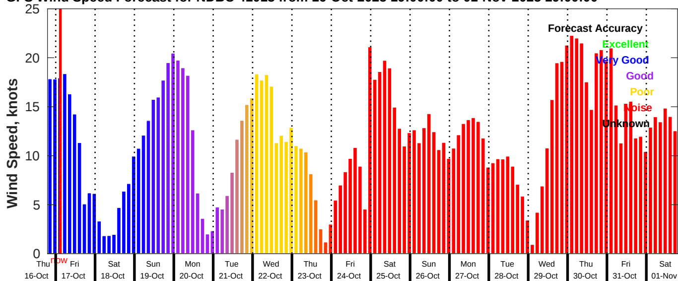
GFS Wind Speed Forecast for NDBC 41013 from 16-Oct-2025 19:00:00 to 01-Nov-2025 19:00:00
