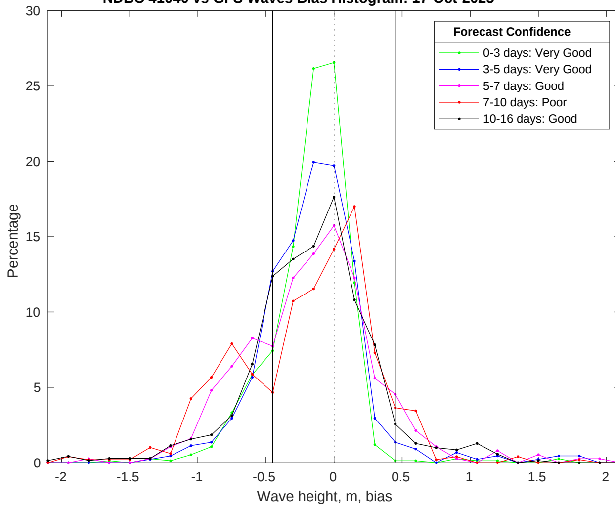
NDBC 41040 vs GFS Waves Bias Histogram: 17-Oct-2025
