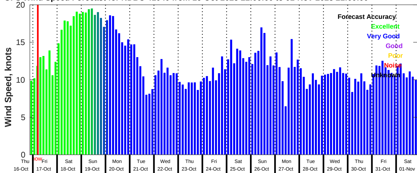
GFS Wind Speed Forecast for NDBC 41040 from 16-Oct-2025 21:00:00 to 01-Nov-2025 21:00:00
