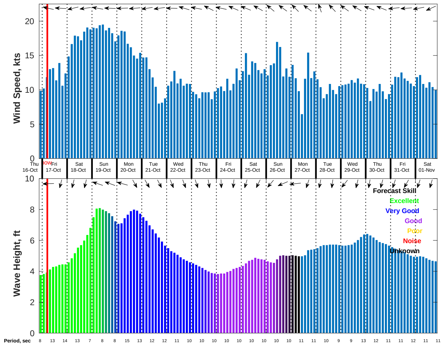
Wind & Wave Forecast for NDBC 41040 from 16-Oct-2025 21:00:00 to 01-Nov-2025 21:00:00
