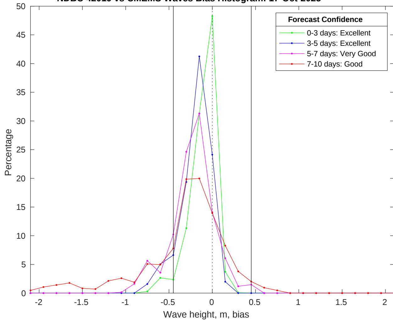
NDBC 42019 vs CMEMS Waves Bias Histogram: 17-Oct-2025
