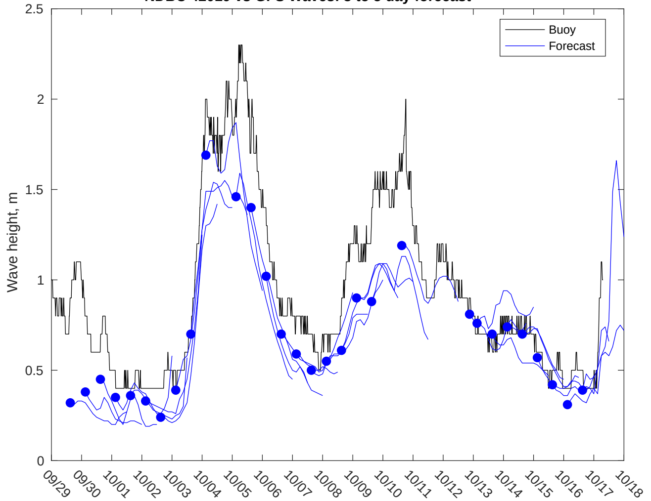
NDBC 42019 vs GFS Waves: 3 to 5 day forecast
