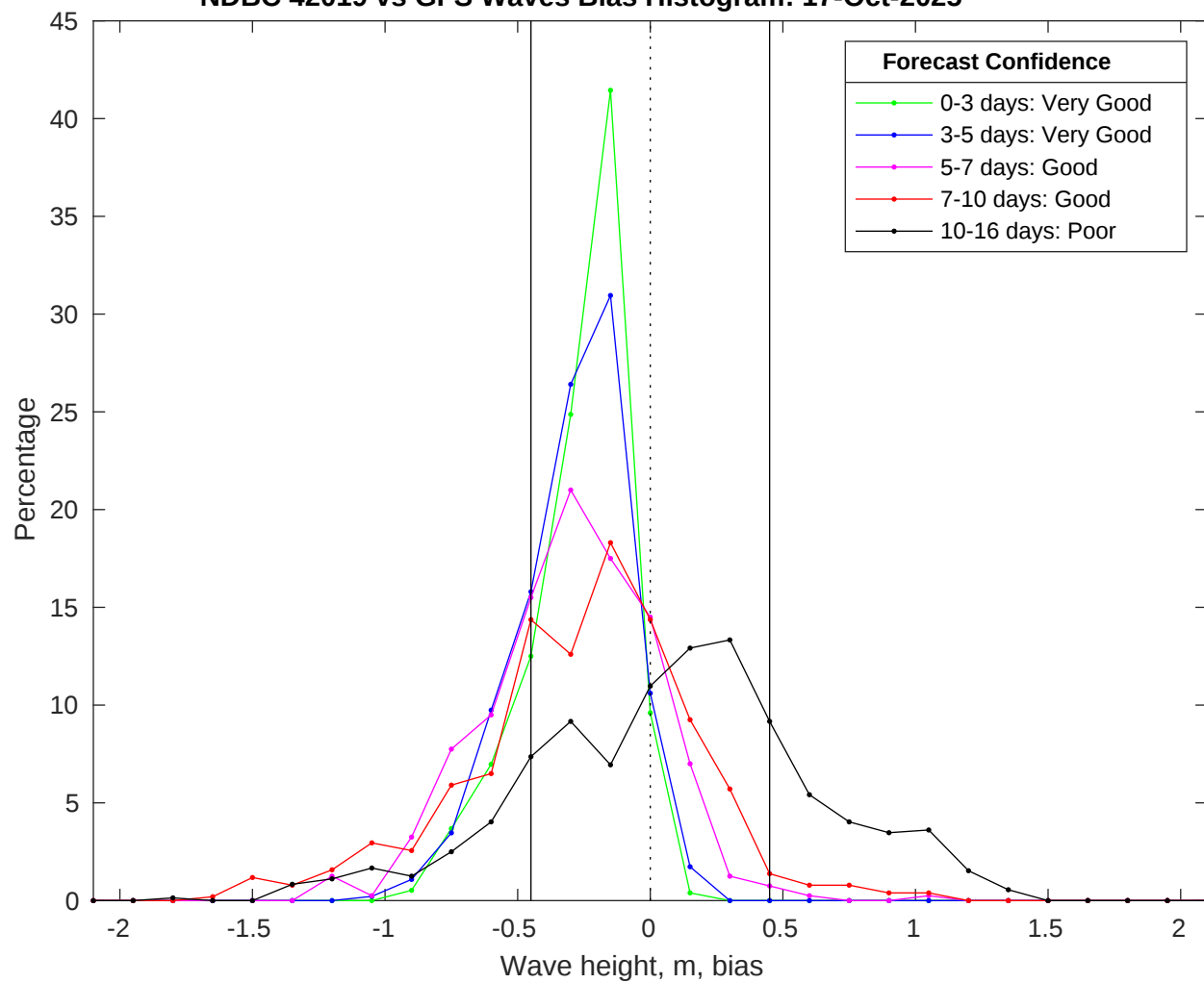
NDBC 42019 vs GFS Waves Bias Histogram: 17-Oct-2025
