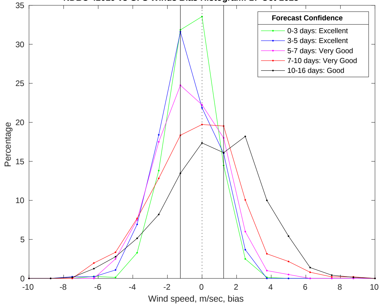
NDBC 42019 vs GFS Winds Bias Histogram: 17-Oct-2025
