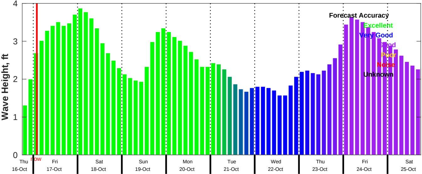
CMEMS Wave Forecast for NDBC 42019 from 16-Oct-2025 18:00:00 to 25-Oct-2025 18:00:00
