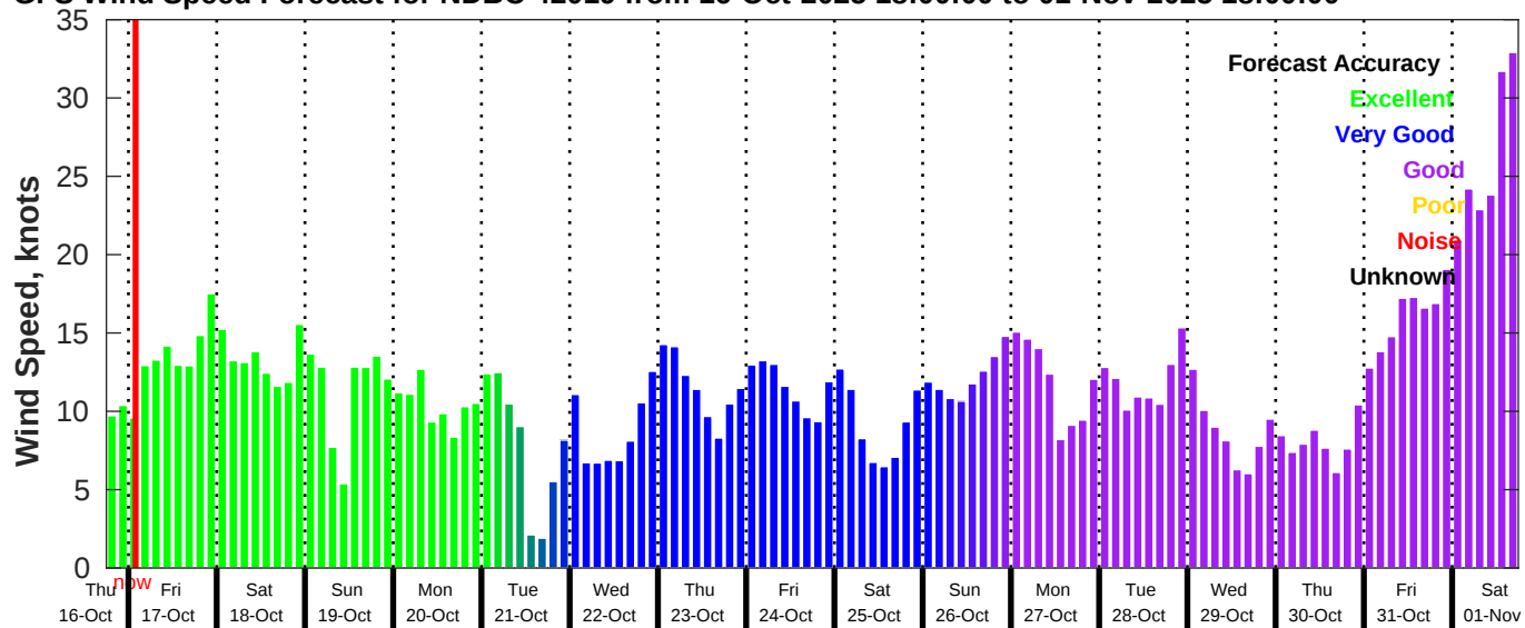
GFS Wind Speed Forecast for NDBC 42019 from 16-Oct-2025 18:00:00 to 01-Nov-2025 18:00:00
