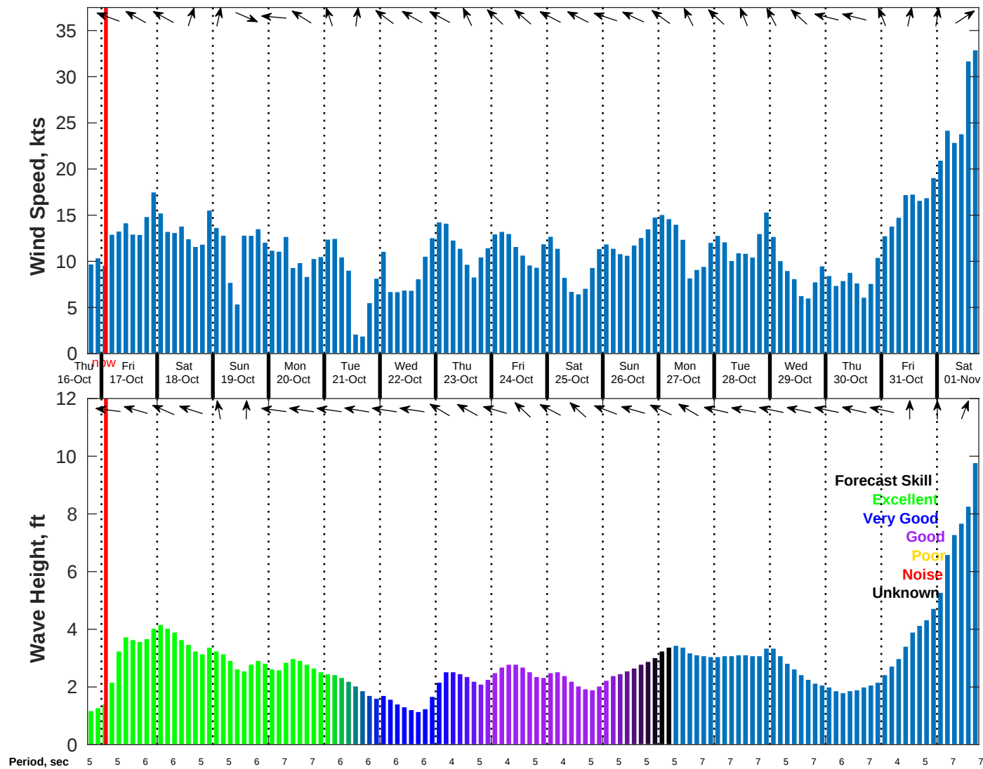
Wind & Wave Forecast for NDBC 42019 from 16-Oct-2025 18:00:00 to 01-Nov-2025 18:00:00
