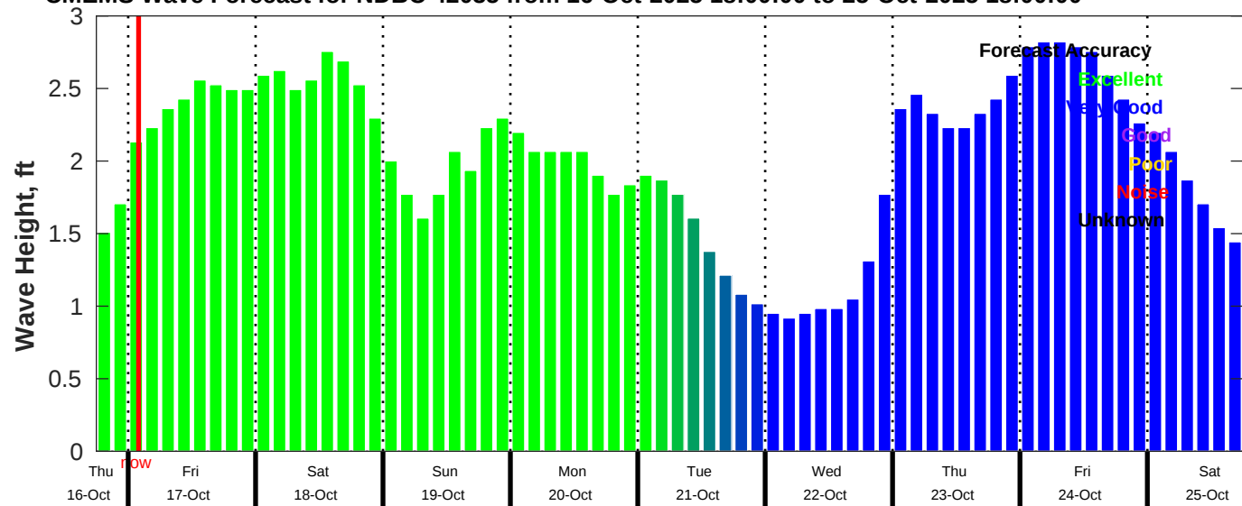
CMEMS Wave Forecast for NDBC 42035 from 16-Oct-2025 18:00:00 to 25-Oct-2025 18:00:00
