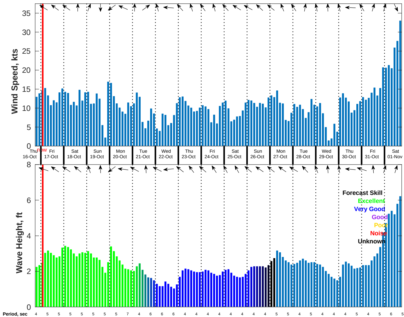
Wind & Wave Forecast for NDBC 42035 from 16-Oct-2025 18:00:00 to 01-Nov-2025 18:00:00
