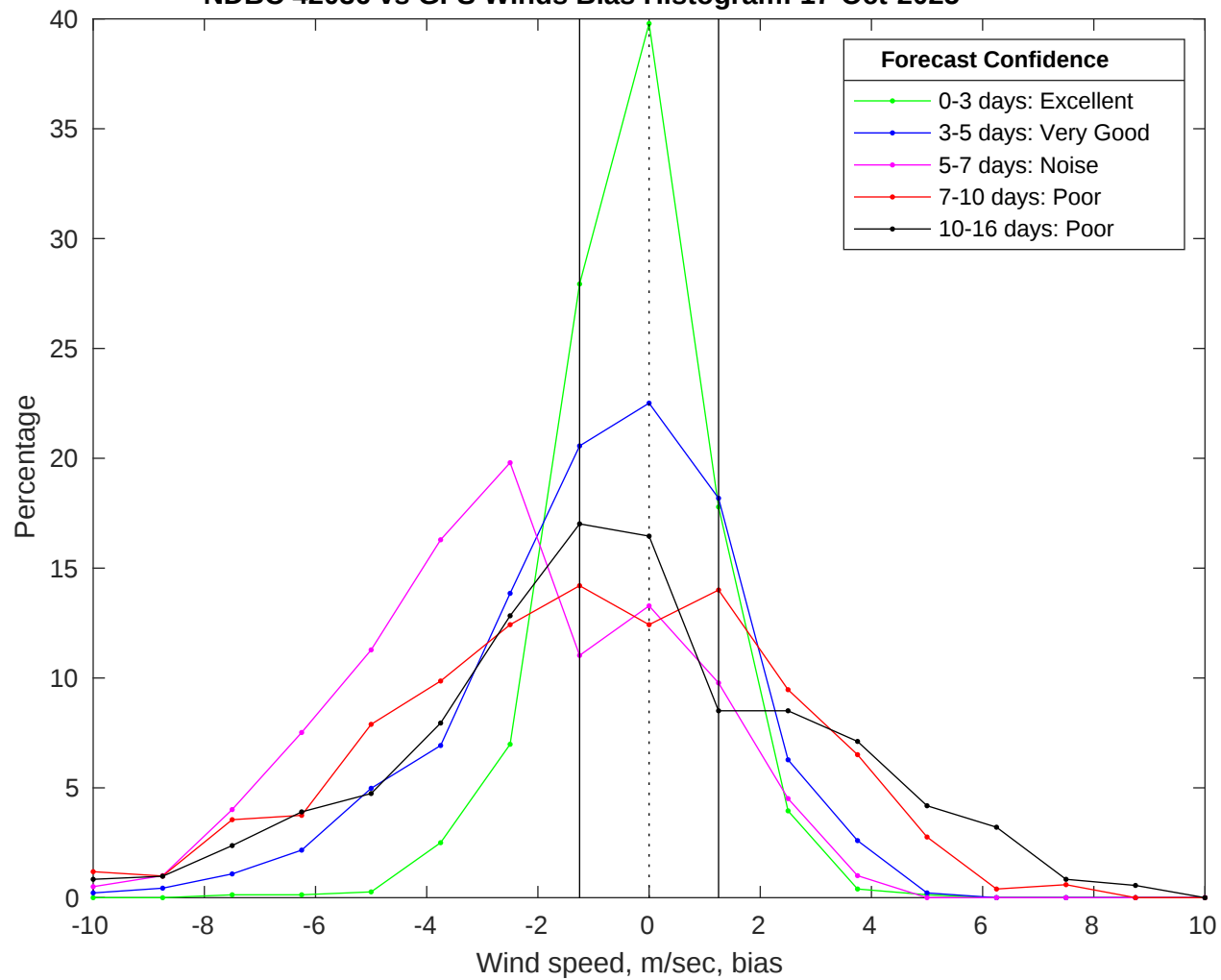
NDBC 42036 vs GFS Winds Bias Histogram: 17-Oct-2025
