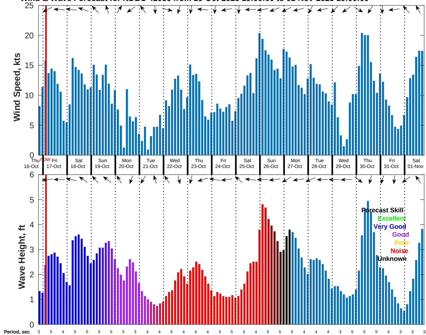
Wind & Wave Forecast for NDBC 42036 from 16-Oct-2025 19:00:00 to 01-Nov-2025 19:00:00
