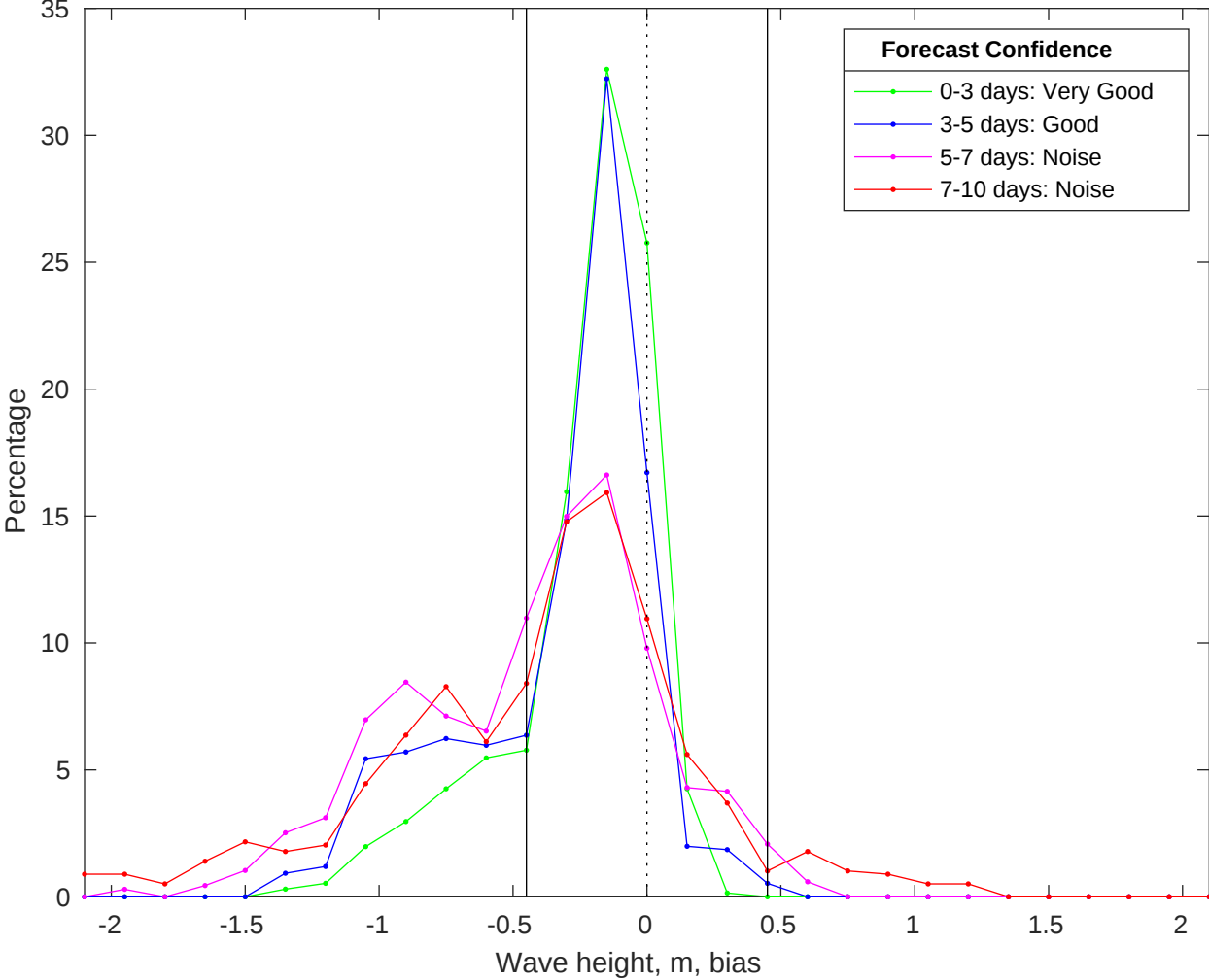
NDBC 42040 vs CMEMS Waves Bias Histogram: 17-Oct-2025
