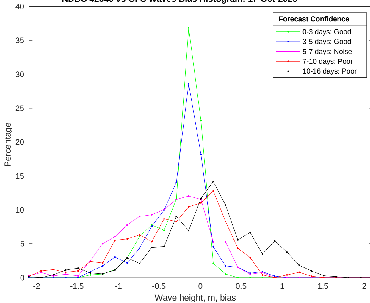
NDBC 42040 vs GFS Waves Bias Histogram: 17-Oct-2025
