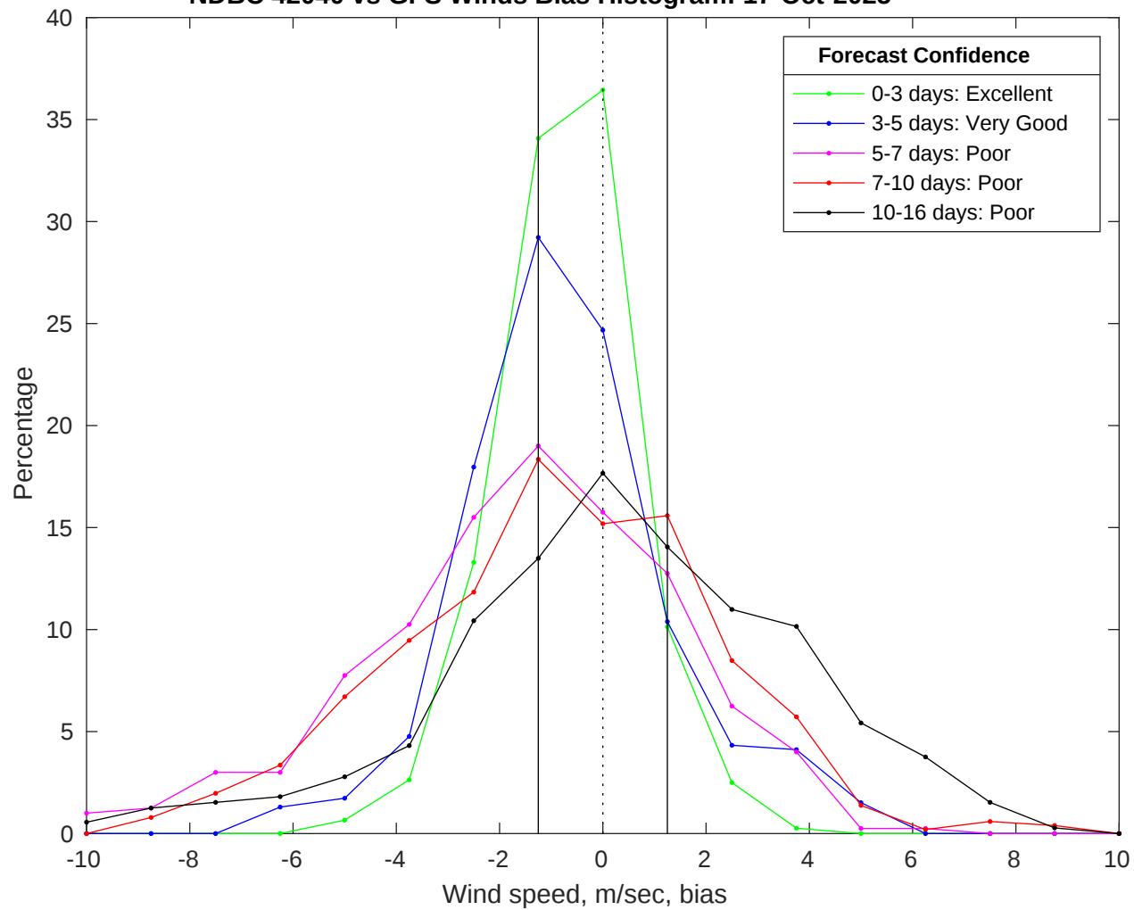
NDBC 42040 vs GFS Winds Bias Histogram: 17-Oct-2025
