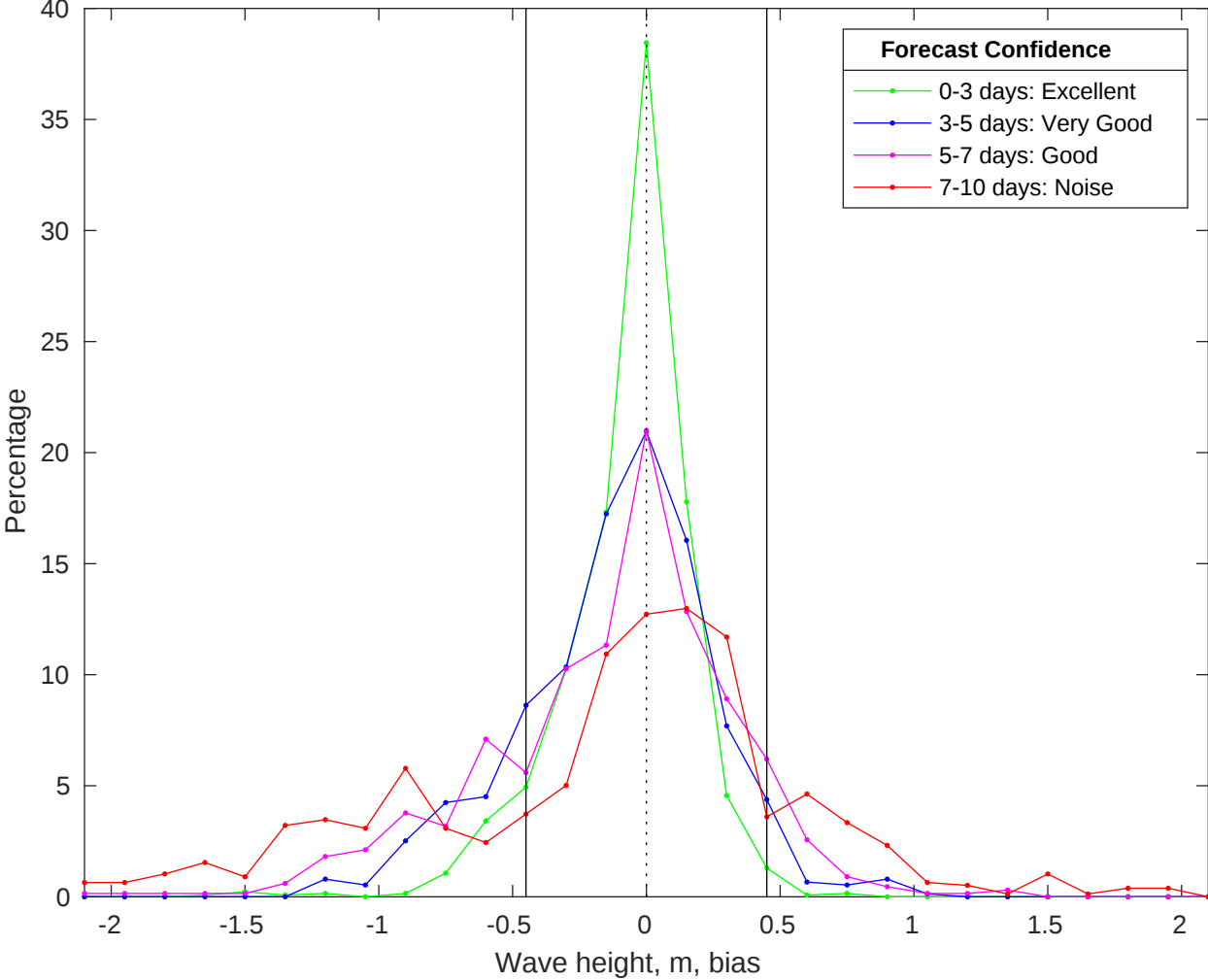
NDBC 44008 vs CMEMS Waves Bias Histogram: 17-Oct-2025
