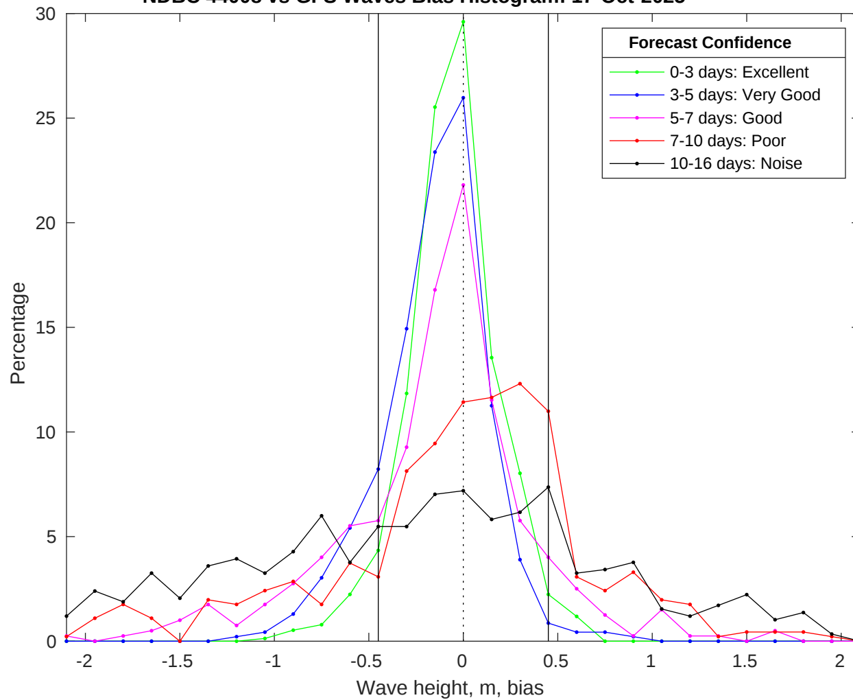
NDBC 44008 vs GFS Waves Bias Histogram: 17-Oct-2025
