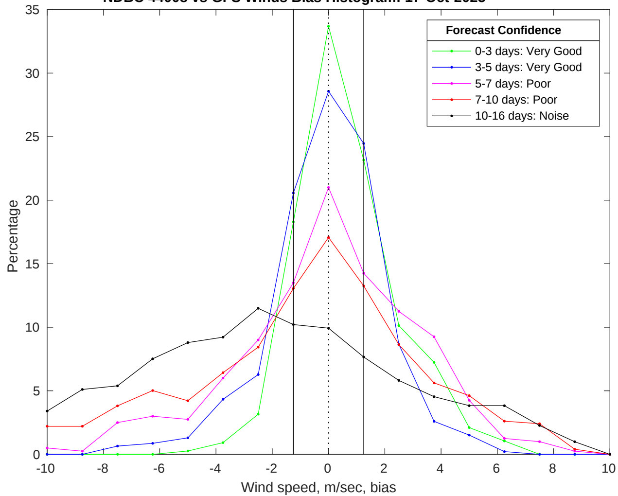
NDBC 44008 vs GFS Winds Bias Histogram: 17-Oct-2025
