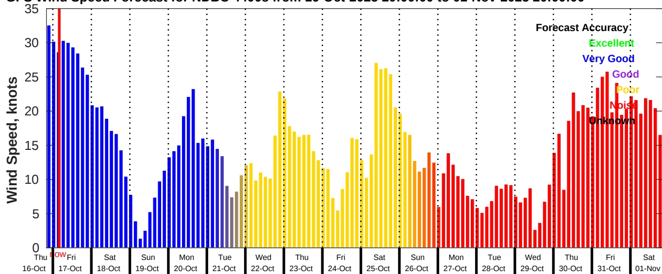
GFS Wind Speed Forecast for NDBC 44008 from 16-Oct-2025 20:00:00 to 01-Nov-2025 20:00:00
