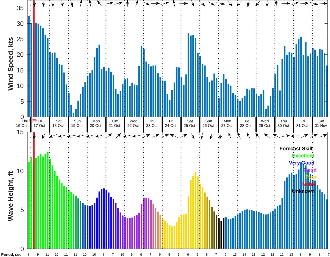
Wind & Wave Forecast for NDBC 44008 from 16-Oct-2025 20:00:00 to 01-Nov-2025 20:00:00
