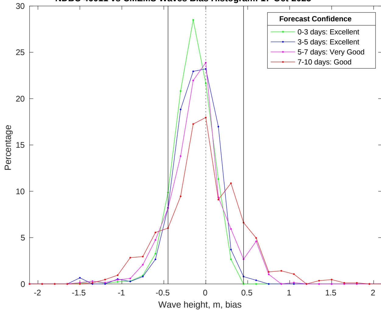
NDBC 46011 vs CMEMS Waves Bias Histogram: 17-Oct-2025
