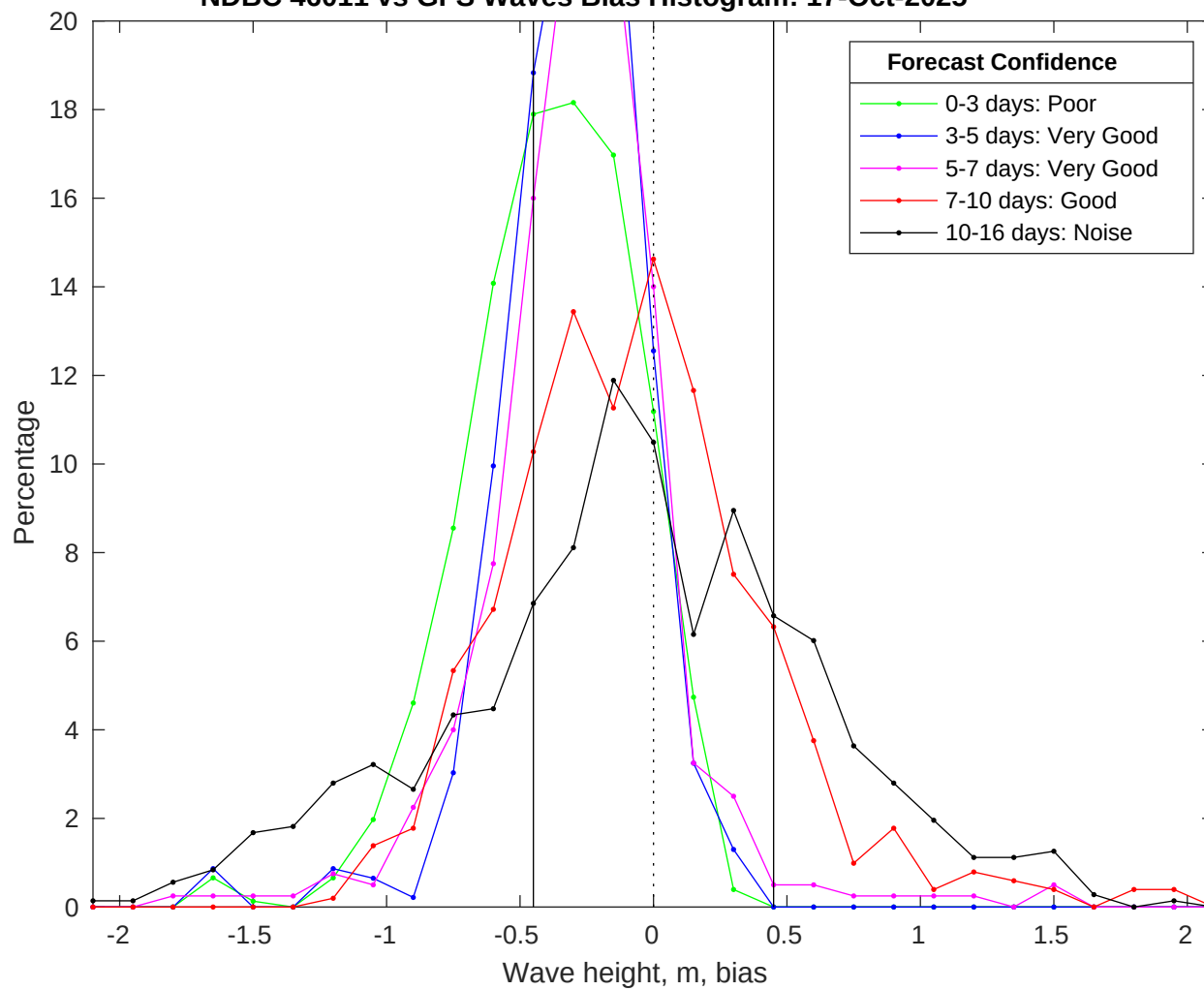
NDBC 46011 vs GFS Waves Bias Histogram: 17-Oct-2025
