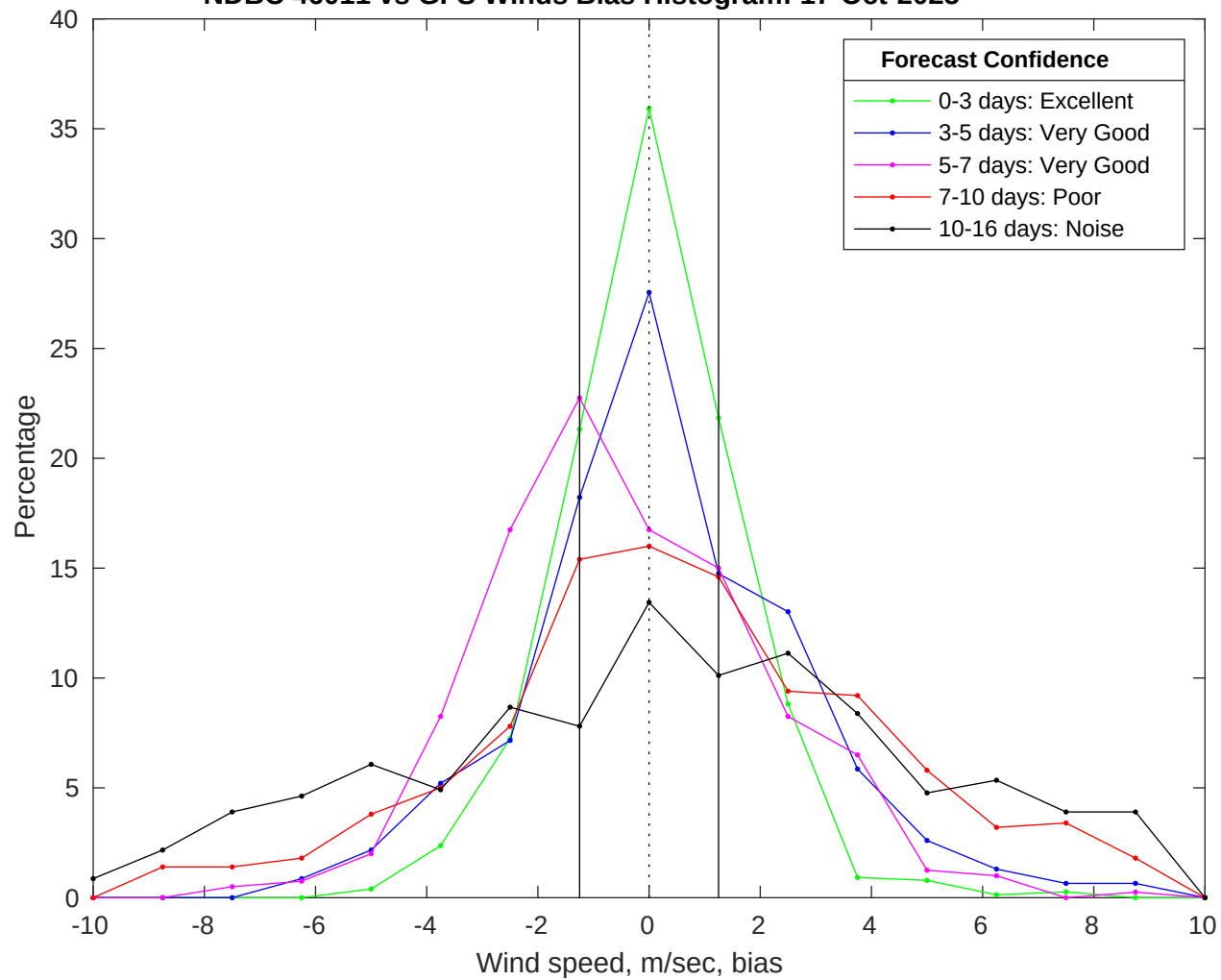
NDBC 46011 vs GFS Winds Bias Histogram: 17-Oct-2025
