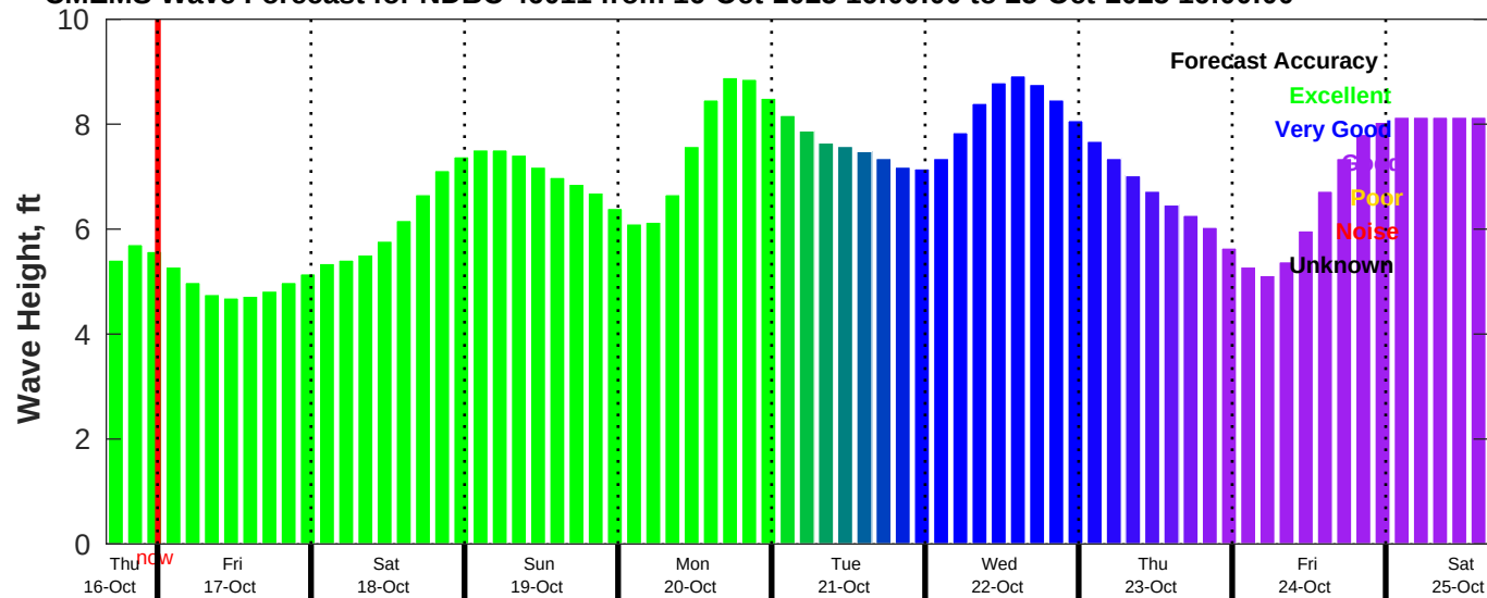
CMEMS Wave Forecast for NDBC 46011 from 16-Oct-2025 16:00:00 to 25-Oct-2025 16:00:00
