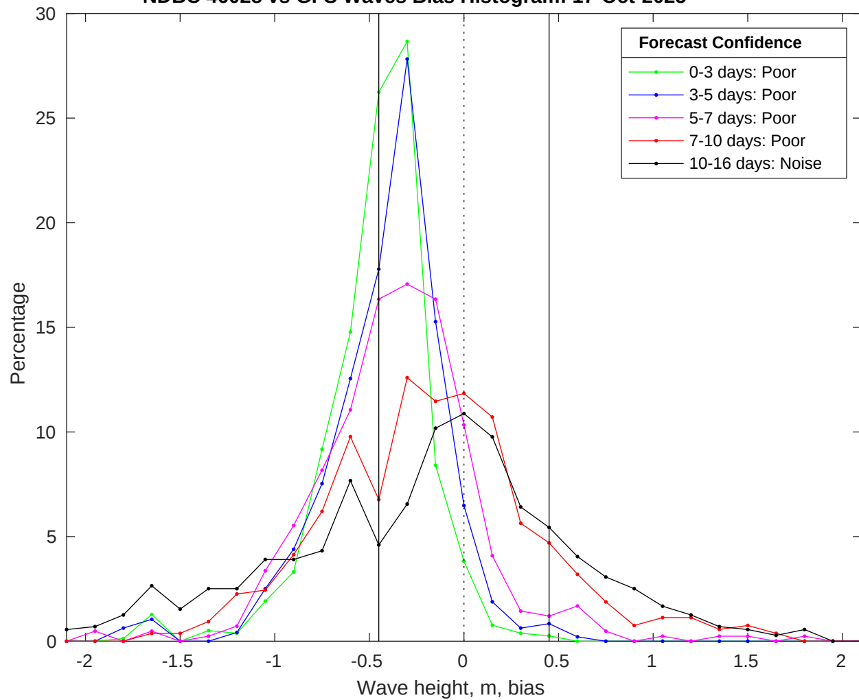
NDBC 46028 vs GFS Waves Bias Histogram: 17-Oct-2025
