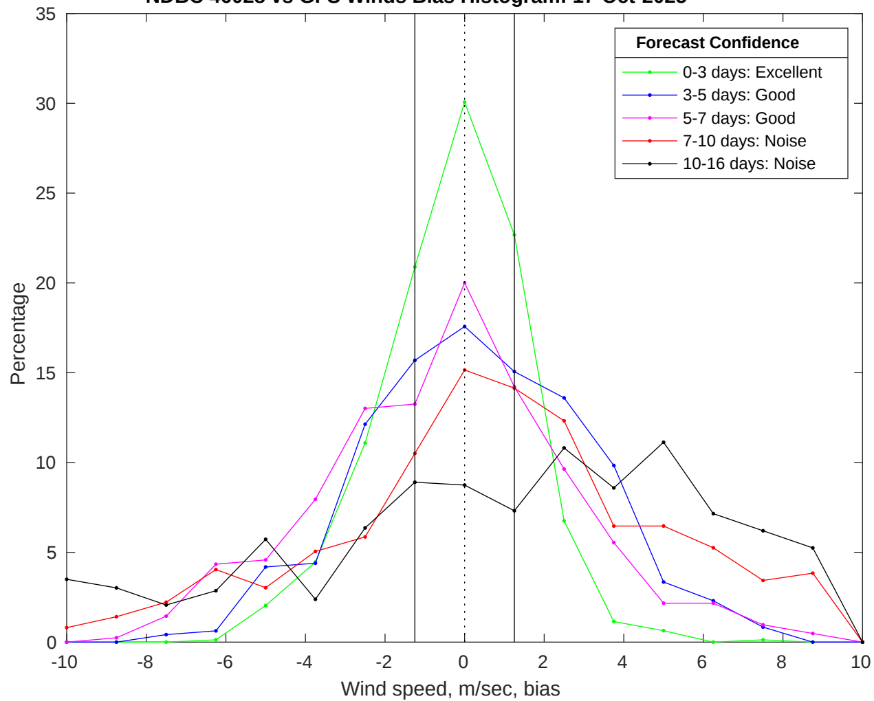
NDBC 46028 vs GFS Winds Bias Histogram: 17-Oct-2025
