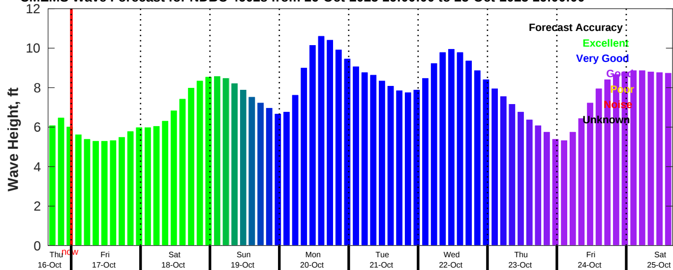
CMEMS Wave Forecast for NDBC 46028 from 16-Oct-2025 16:00:00 to 25-Oct-2025 16:00:00
