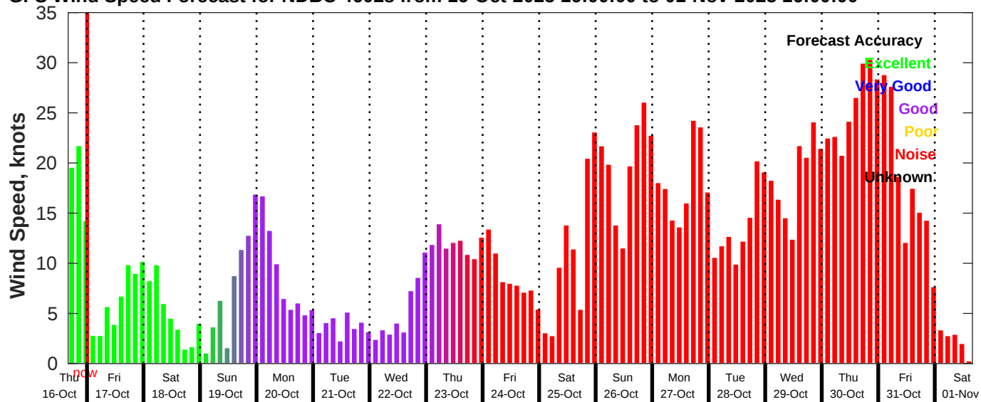
GFS Wind Speed Forecast for NDBC 46028 from 16-Oct-2025 16:00:00 to 01-Nov-2025 16:00:00
