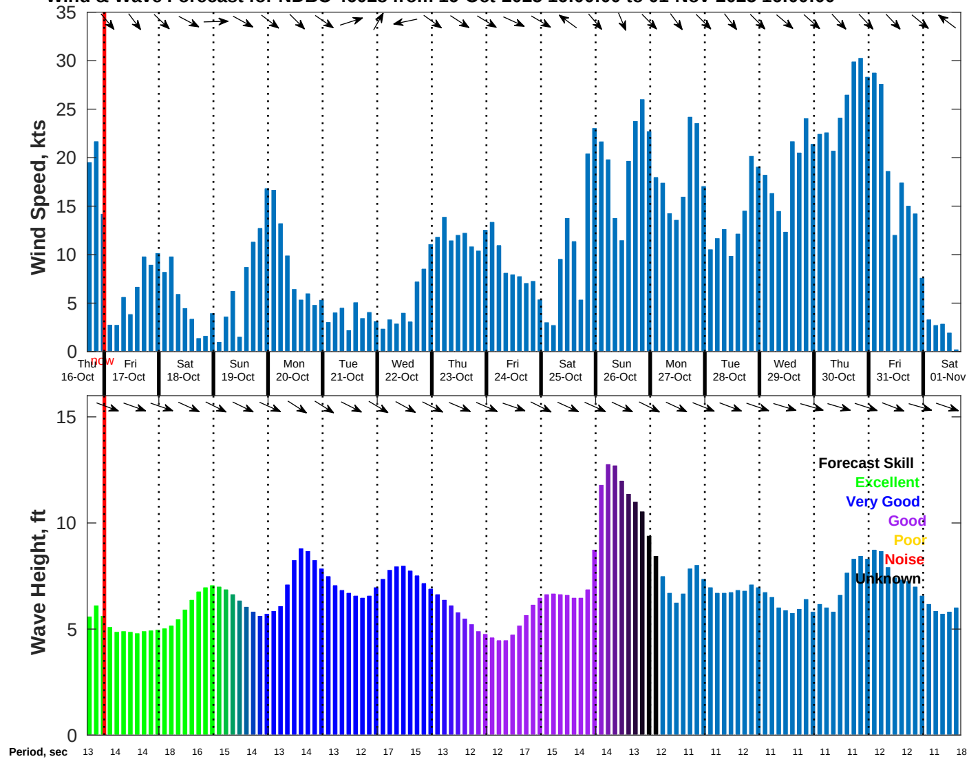
Wind & Wave Forecast for NDBC 46028 from 16-Oct-2025 16:00:00 to 01-Nov-2025 16:00:00
